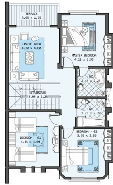
First Floor 120 m 2
