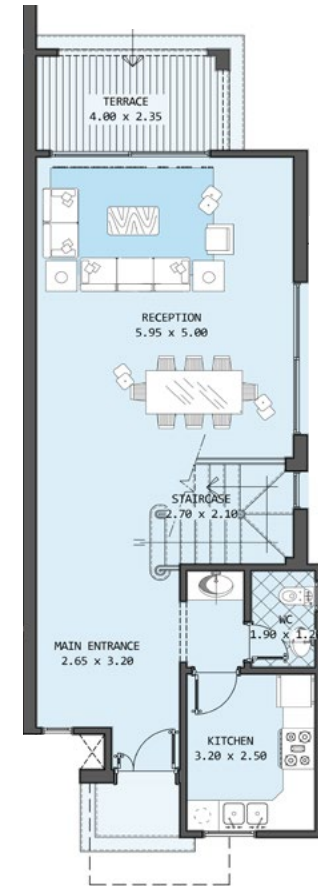
Ground Plan 89 M 2
